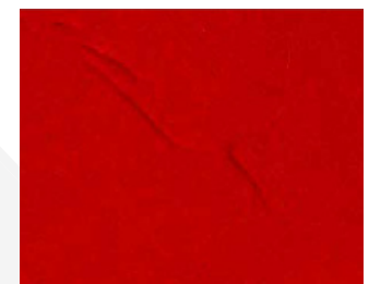
Red Giant
