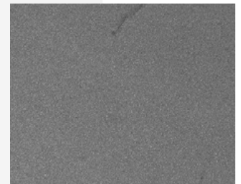
Moon Crater
