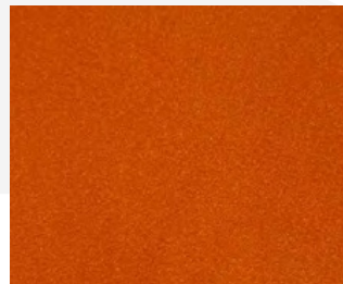
Cosmic Dust
