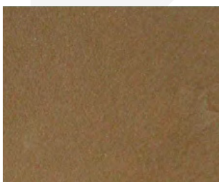
Saturn's Rings
