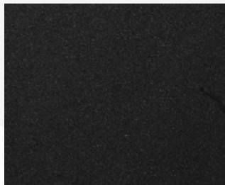
Cosmic Black
