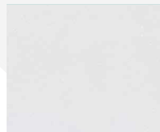
Polaris White
